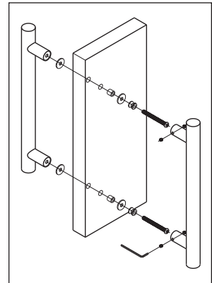
D. Back-To-Back Mounting
