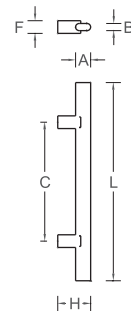
Model A B F H C DPD4004 38mm 18mm ∅ 32mm 83mm Per project spec DPD4005 45mm 25mm ∅ 38mm 90mm Per project spec
